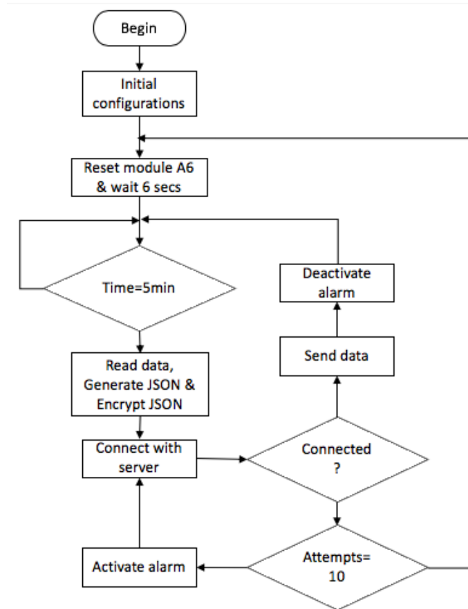
Figure 2. Flowchart used to describe microcontroller activities.
