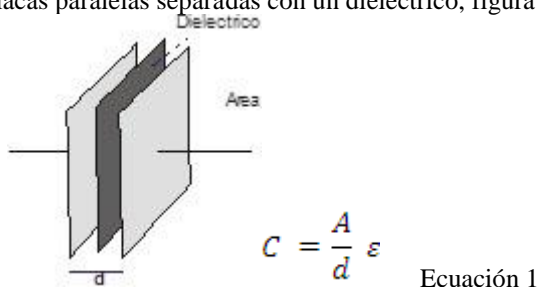
Figura 1. Capacitor simple.
