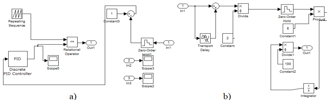
Figure 2. Block diagram of a 3 states PI controller and state of charge stimator.
