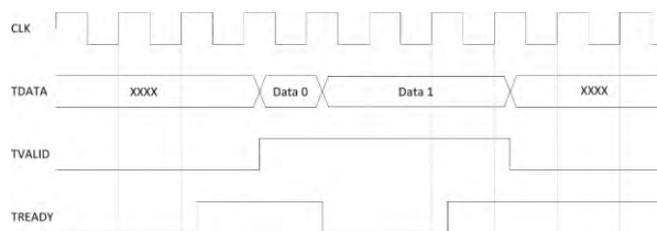
Figure 4. 12 Handshake AXI4-Stream.
