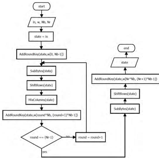
Figure 2. 11 Flowchart AES.
