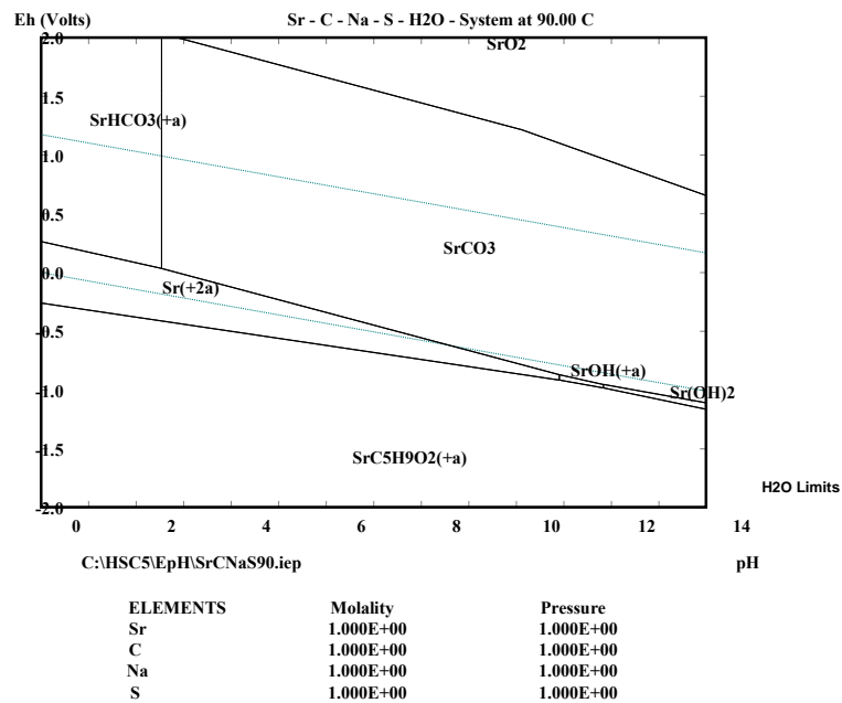
Figura 3. Diagrama HSC (Eh-pH)
