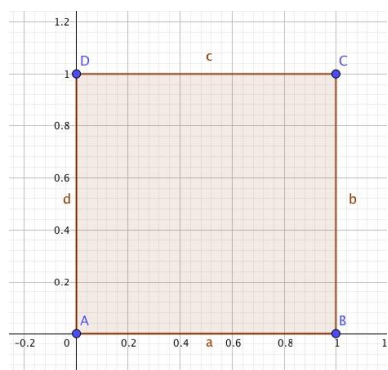
Figura 3. A = b * f(b) = 1
