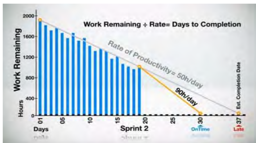
Figura 1. Burndown Chart
