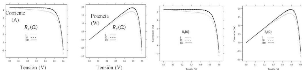
Perpiñán Lamigueiro, 2015
